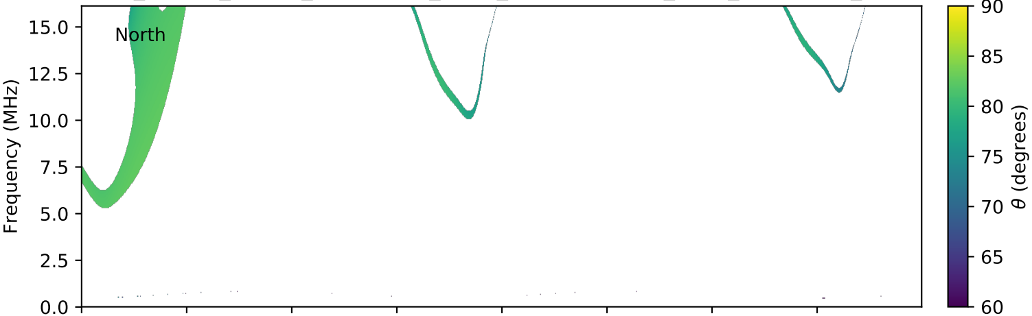
expres_cassini_jupiter_ganymede_isaac_lossc-wid1deg_3kev_20011128_v01.cdf
