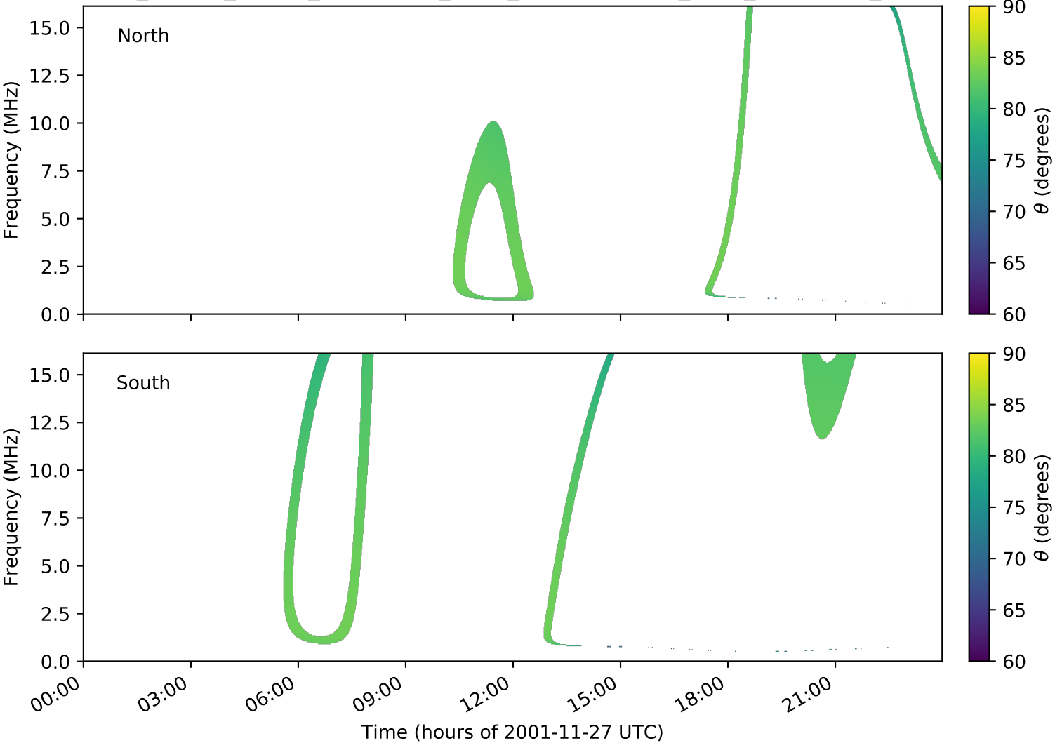
expres_cassini_jupiter_ganymede_isaac_lossc-wid1deg_3kev_20011127_v01.cdf
