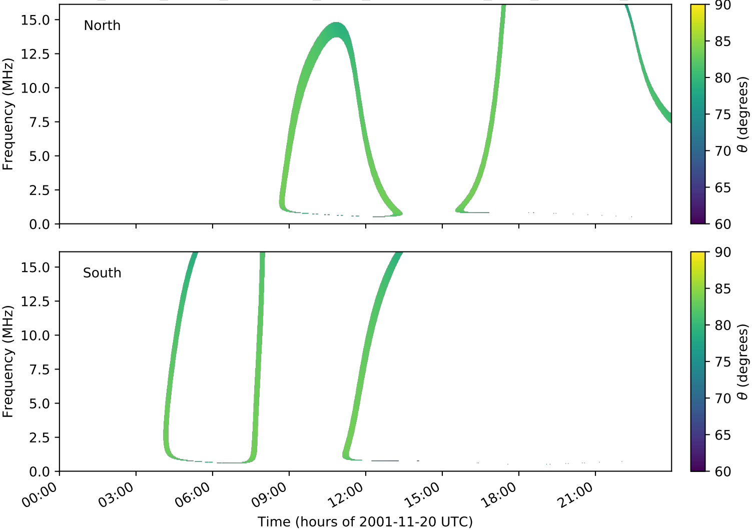
expres_cassini_jupiter_ganymede_isaac_lossc-wid1deg_3kev_20011120_v01.cdf
