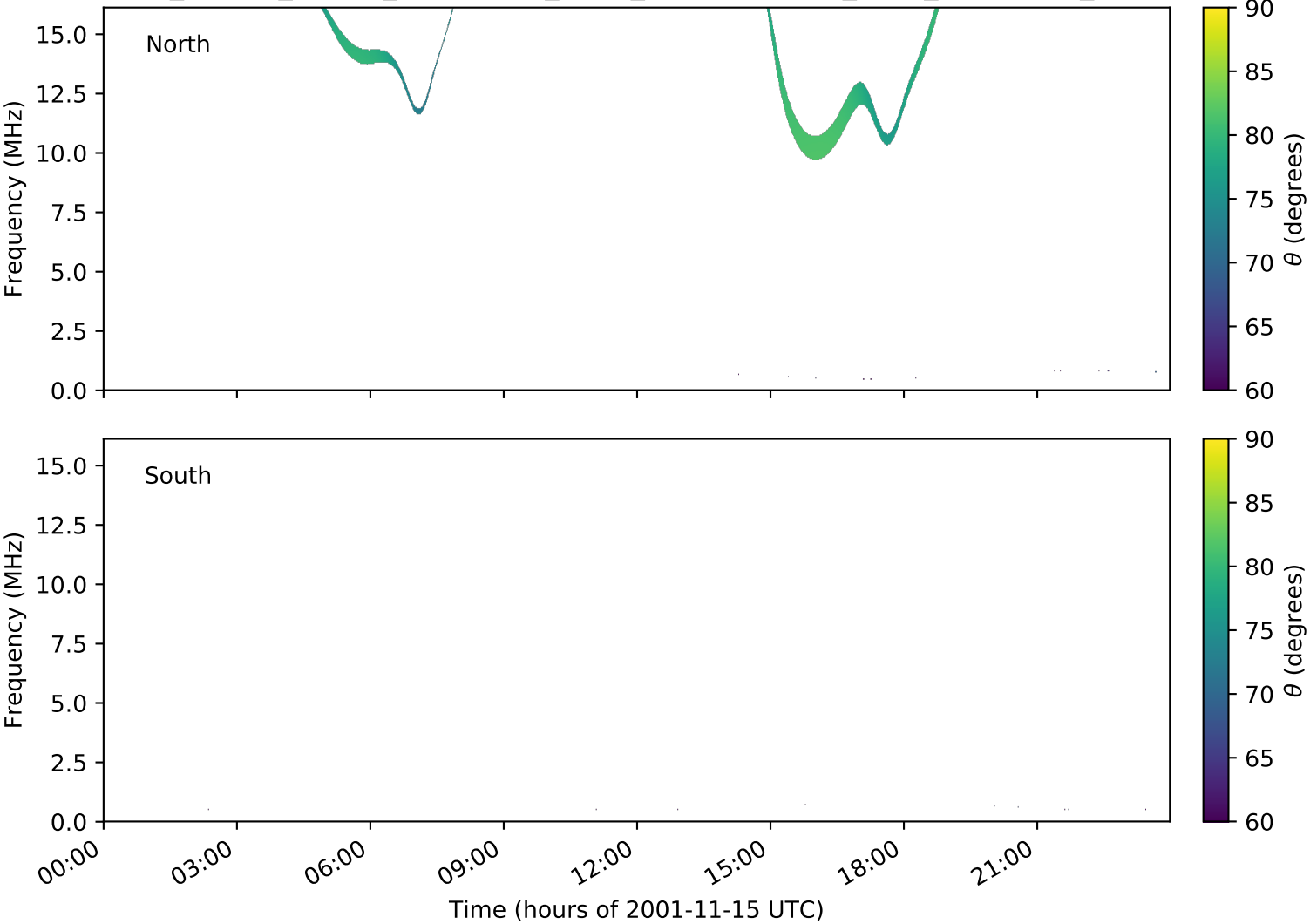
expres_cassini_jupiter_ganymede_isaac_lossc-wid1deg_3kev_20011115_v01.cdf
