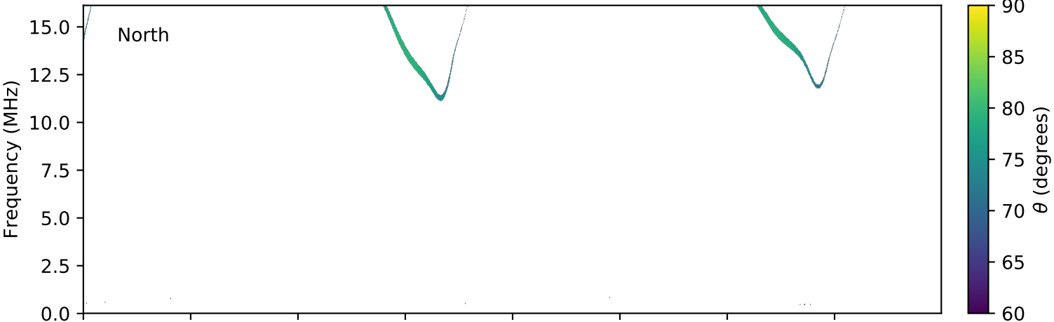
expres_cassini_jupiter_ganymede_isaac_lossc-wid1deg_3kev_20011114_v01.cdf
