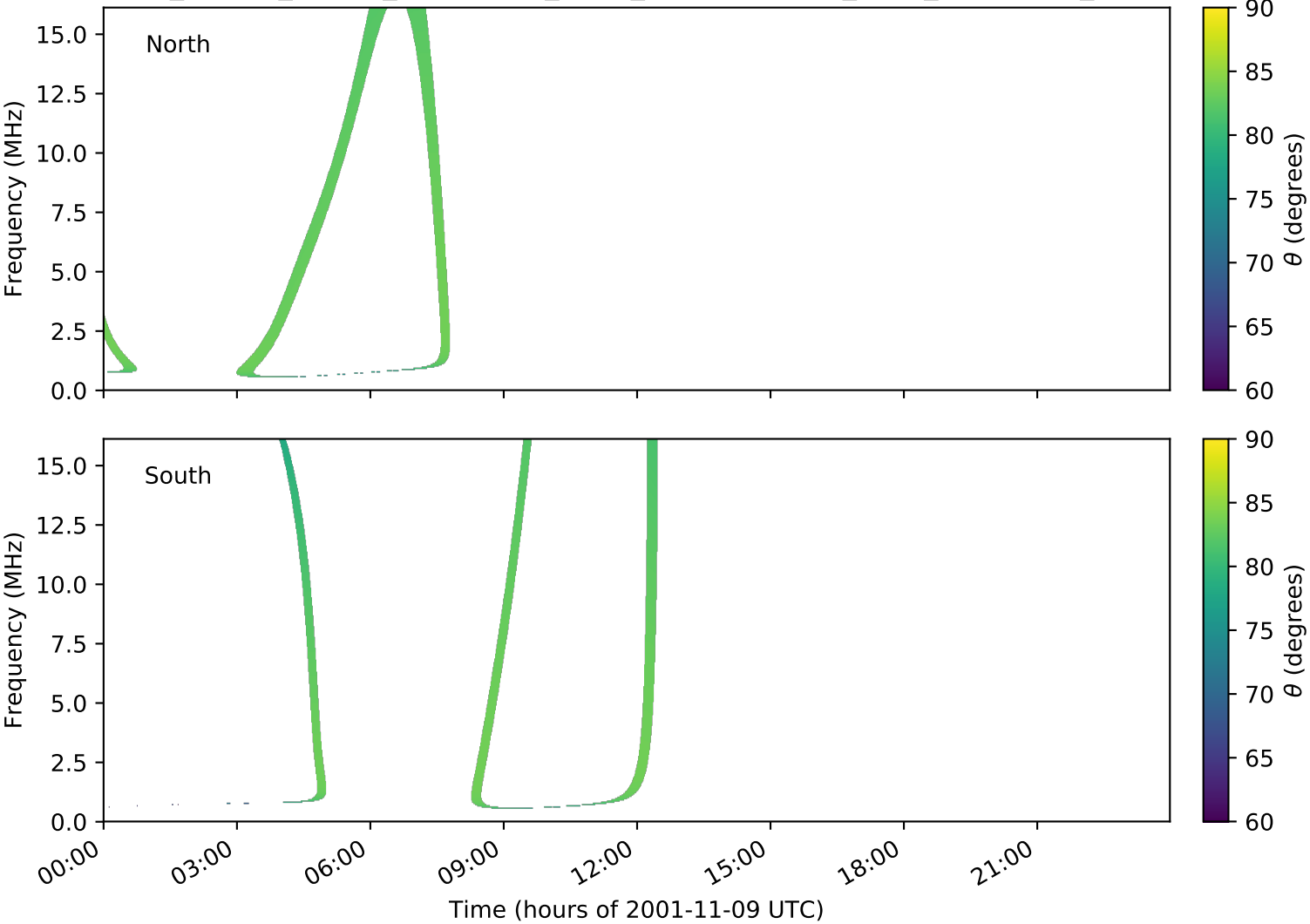
expres_cassini_jupiter_ganymede_isaac_lossc-wid1deg_3kev_20011109_v01.cdf
