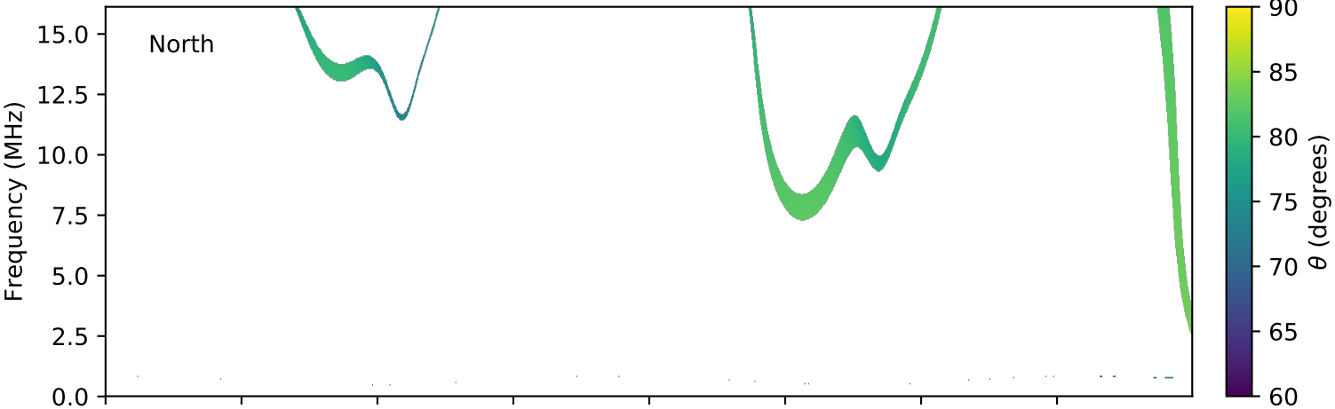
expres_cassini_jupiter_ganymede_isaac_lossc-wid1deg_3kev_20011108_v01.cdf
