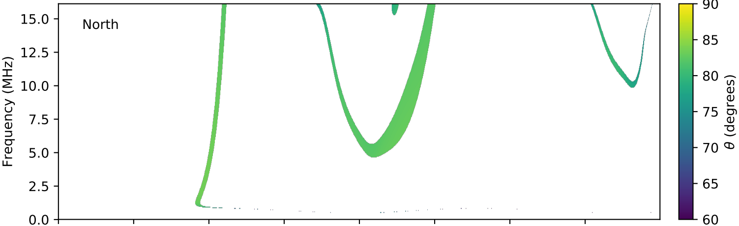
expres_cassini_jupiter_ganymede_isaac_lossc-wid1deg_3kev_20011106_v01.cdf
