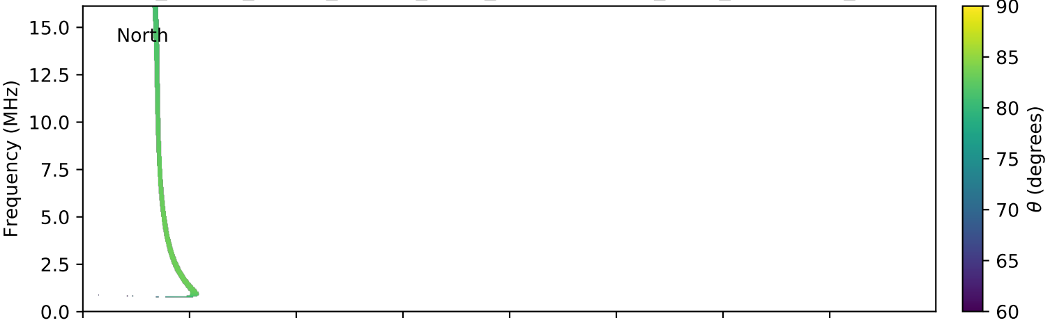
expres_cassini_jupiter_europa_isaac_lossc-wid1deg_3kev_20011130_v01.cdf
