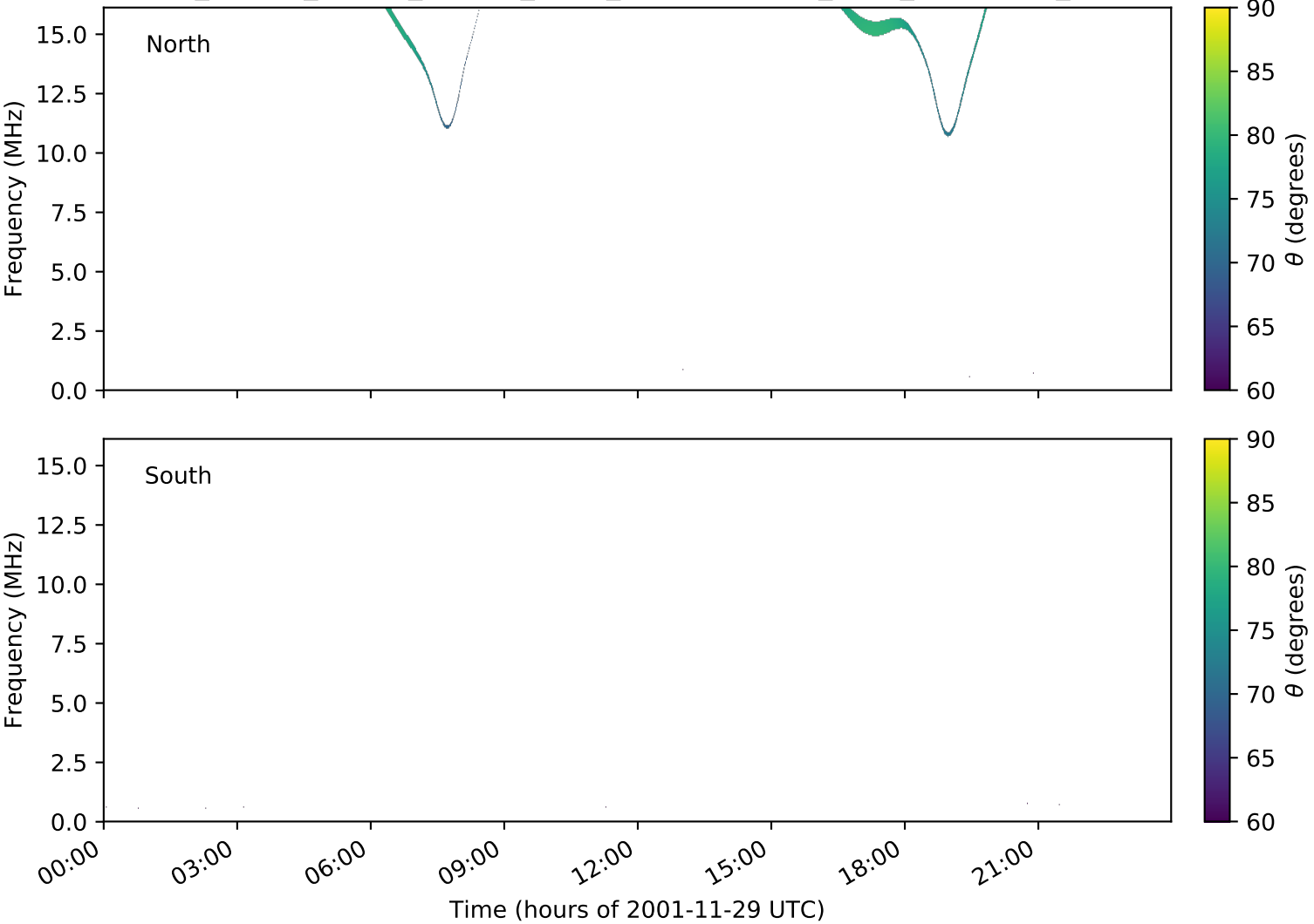
expres_cassini_jupiter_europa_isaac_lossc-wid1deg_3kev_20011129_v01.cdf
