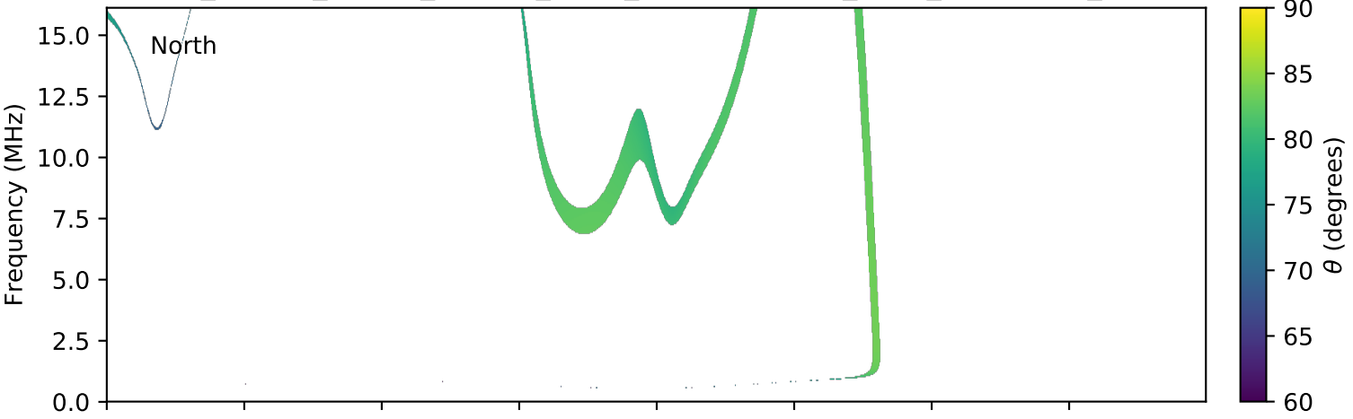
expres_cassini_jupiter_europa_isaac_lossc-wid1deg_3kev_20011126_v01.cdf
