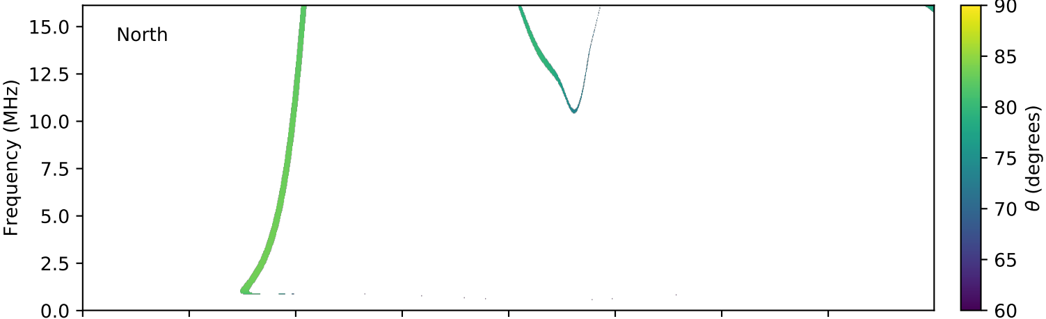
expres_cassini_jupiter_europa_isaac_lossc-wid1deg_3kev_20011125_v01.cdf
