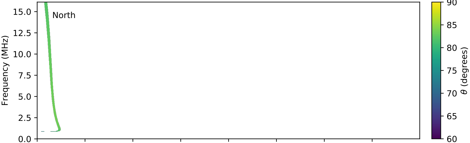
expres_cassini_jupiter_europa_isaac_lossc-wid1deg_3kev_20011123_v01.cdf
