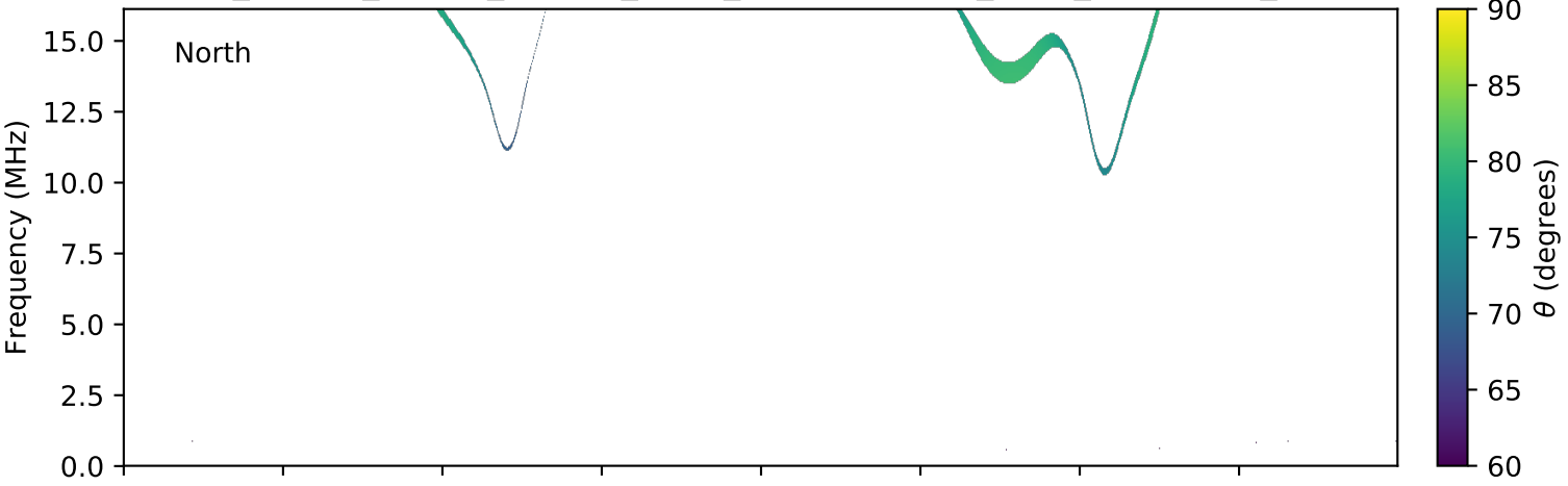
expres_cassini_jupiter_europa_isaac_lossc-wid1deg_3kev_20011122_v01.cdf
