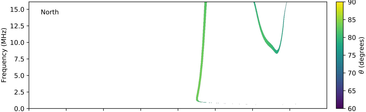
expres_cassini_jupiter_europa_isaac_lossc-wid1deg_3kev_20011121_v01.cdf
