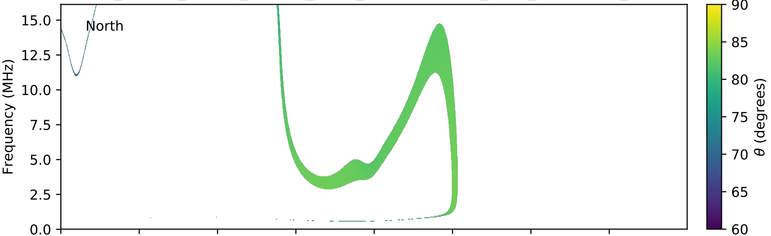
expres_cassini_jupiter_europa_isaac_lossc-wid1deg_3kev_20011119_v01.cdf
