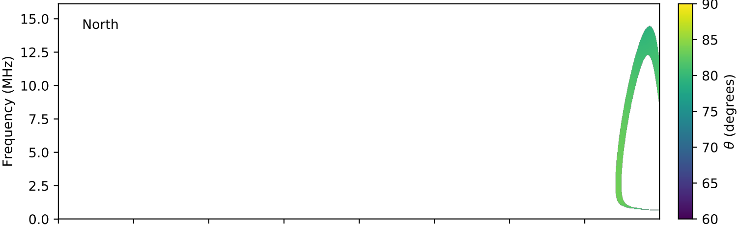
expres_cassini_jupiter_europa_isaac_lossc-wid1deg_3kev_20011117_v01.cdf
