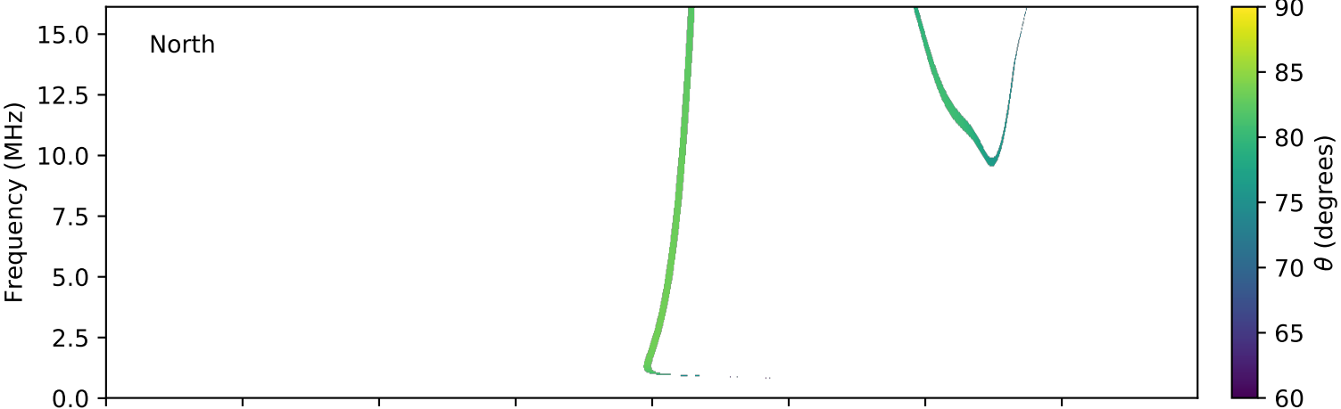
expres_cassini_jupiter_europa_isaac_lossc-wid1deg_3kev_20011114_v01.cdf
