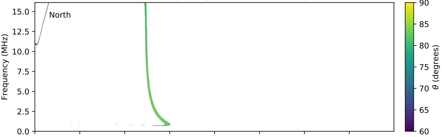
expres_cassini_jupiter_europa_isaac_lossc-wid1deg_3kev_20011112_v01.cdf
