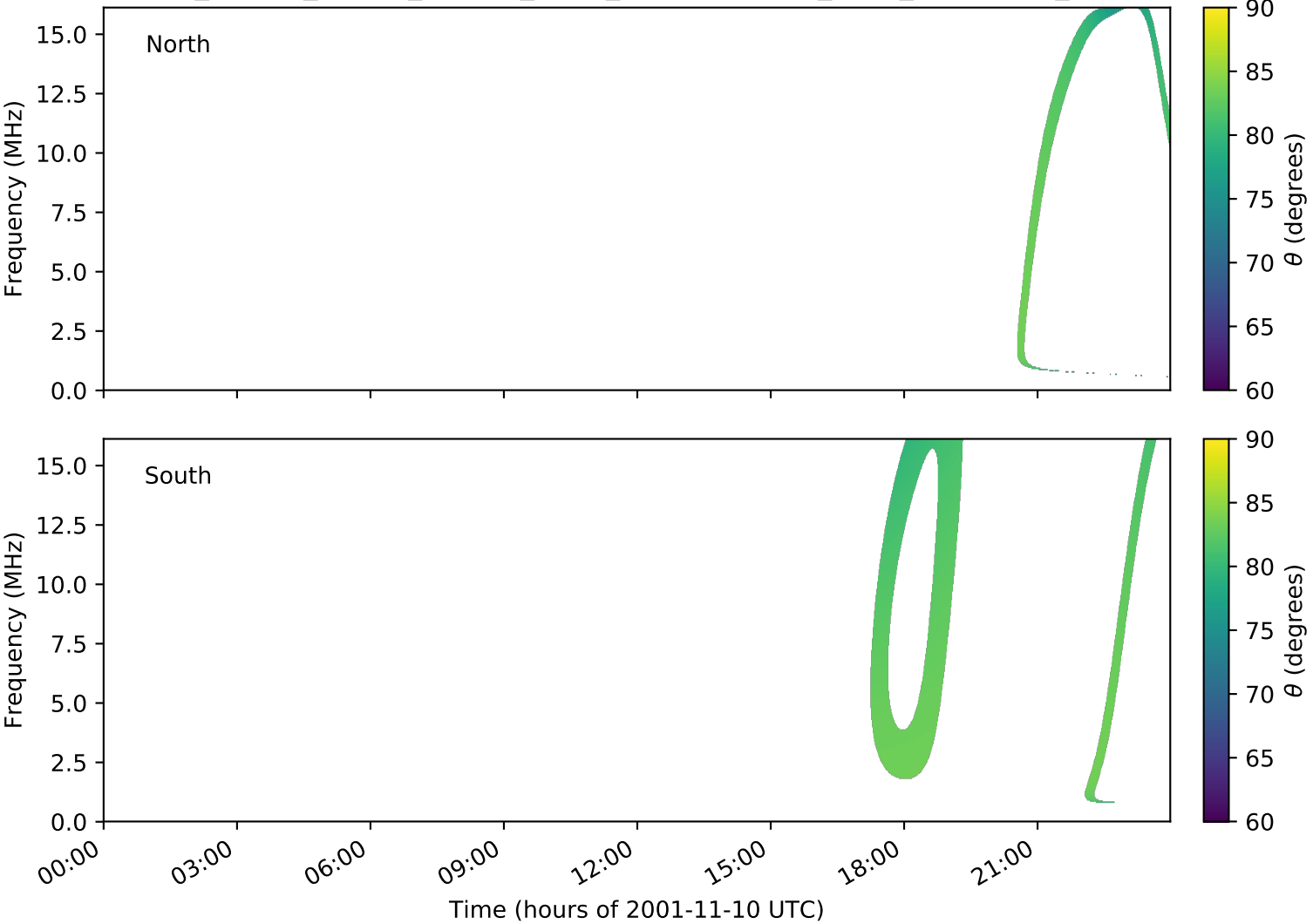
expres_cassini_jupiter_europa_isaac_lossc-wid1deg_3kev_20011110_v01.cdf
