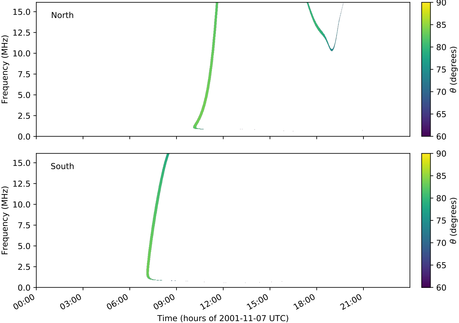
expres_cassini_jupiter_europa_isaac_lossc-wid1deg_3kev_20011107_v01.cdf
