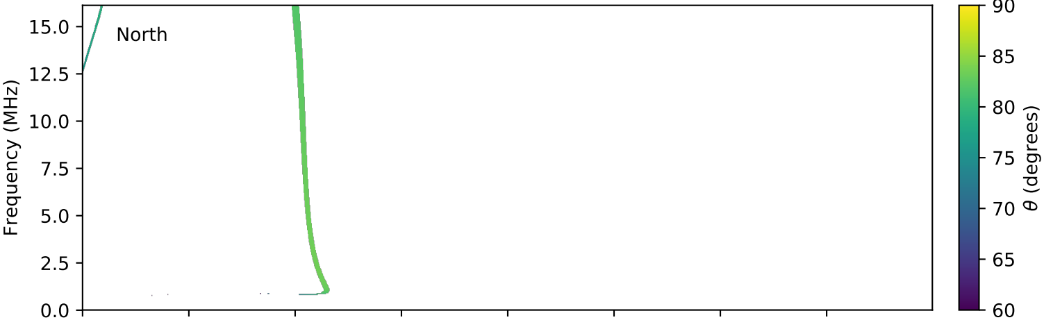
expres_cassini_jupiter_europa_isaac_lossc-wid1deg_3kev_20011105_v01.cdf
