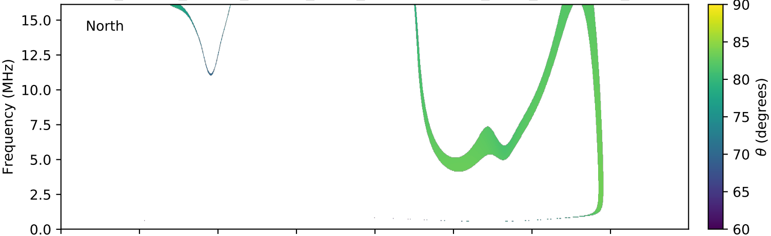
expres_cassini_jupiter_europa_isaac_lossc-wid1deg_3kev_20011101_v01.cdf
