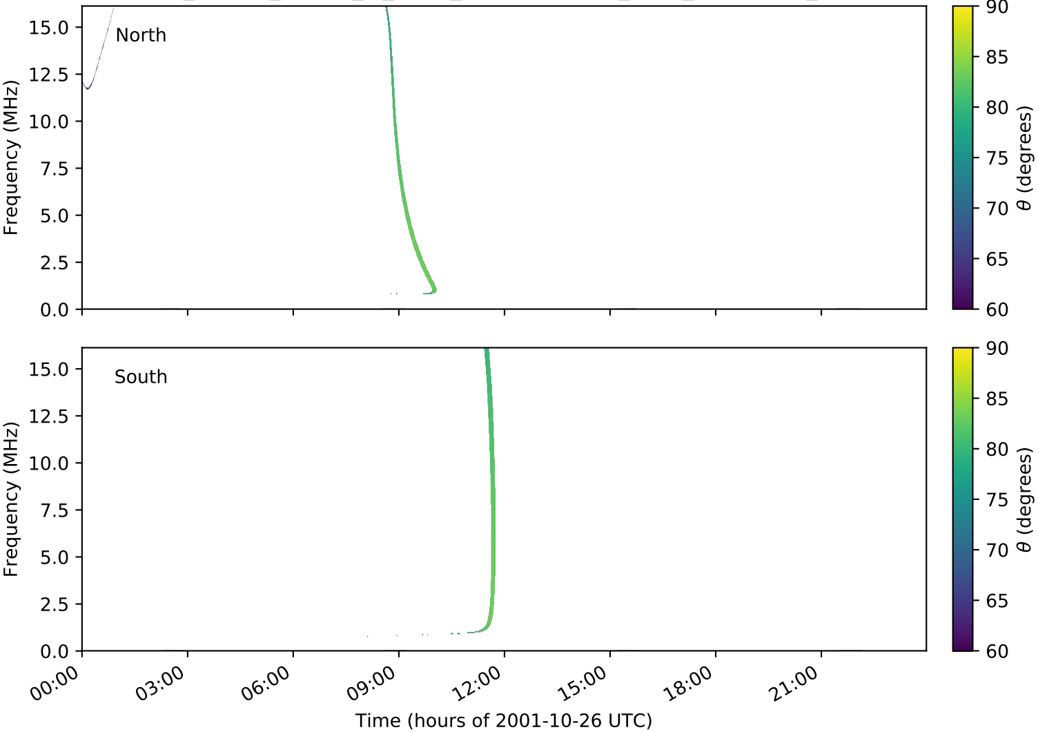
expres_cassini_jupiter_io_isaac_lossc-wid1deg_3kev_20011026_v01.cdf
