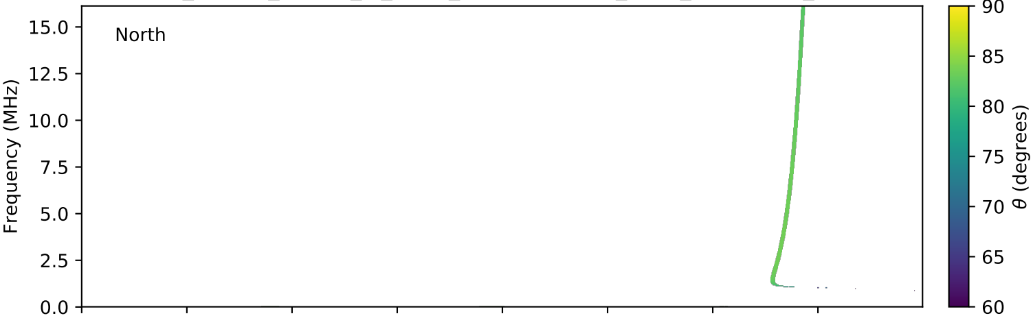
expres_cassini_jupiter_io_isaac_lossc-wid1deg_3kev_20010531_v01.cdf
