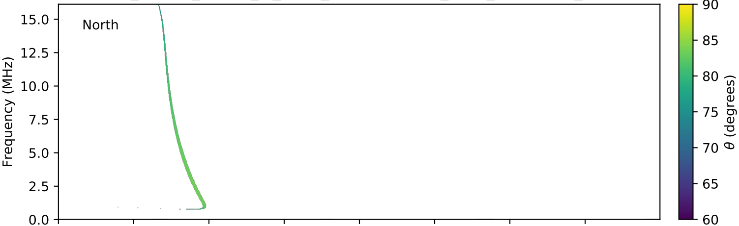
expres_cassini_jupiter_io_isaac_lossc-wid1deg_3kev_20010527_v01.cdf
