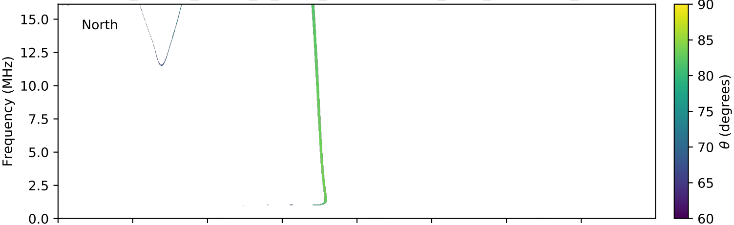
expres_cassini_jupiter_io_isaac_lossc-wid1deg_3kev_20010518_v01.cdf
