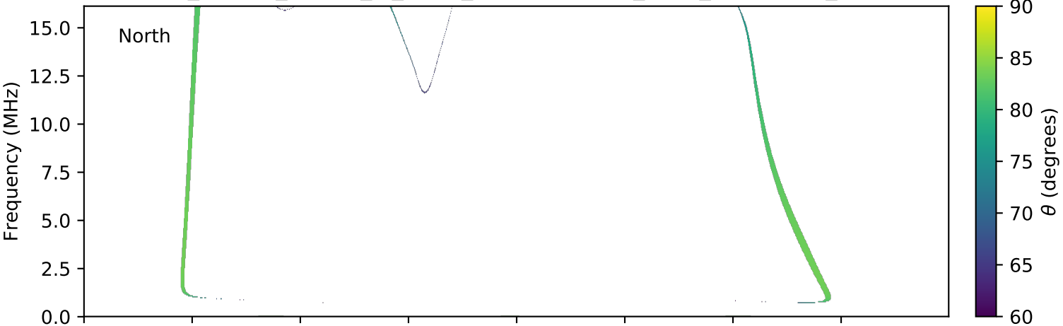
expres_cassini_jupiter_io_isaac_lossc-wid1deg_3kev_20010514_v01.cdf
