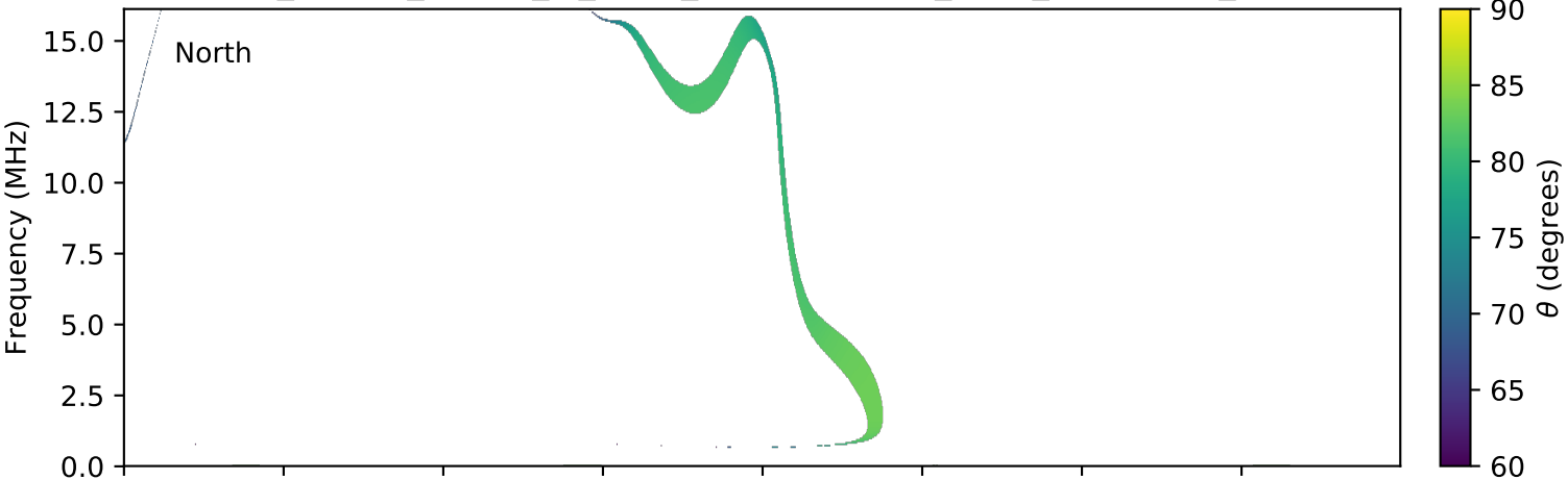
expres_cassini_jupiter_io_isaac_lossc-wid1deg_3kev_20010509_v01.cdf
