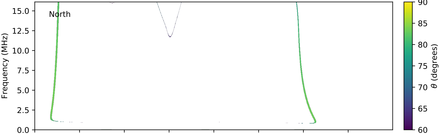
expres_cassini_jupiter_io_isaac_lossc-wid1deg_3kev_20010507_v01.cdf
