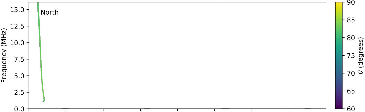
expres_cassini_jupiter_io_isaac_lossc-wid1deg_3kev_20010506_v01.cdf
