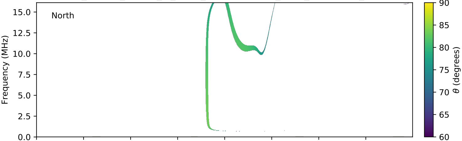
expres_cassini_jupiter_io_isaac_lossc-wid1deg_3kev_20010503_v01.cdf
