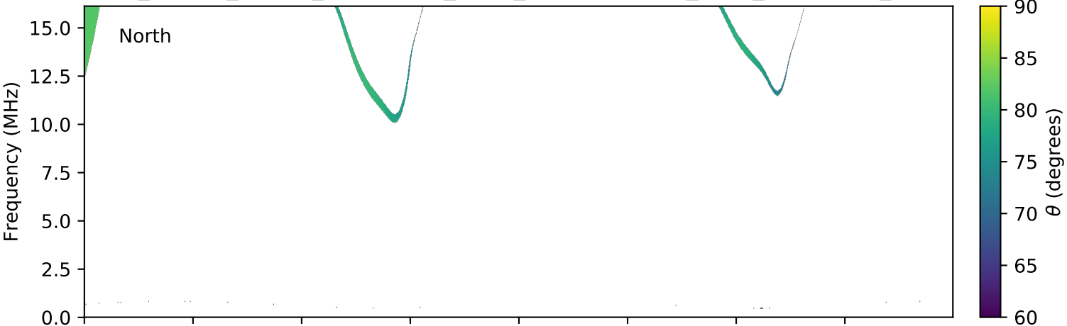
expres_cassini_jupiter_ganymede_isaac_lossc-wid1deg_3kev_20010526_v01.cdf
