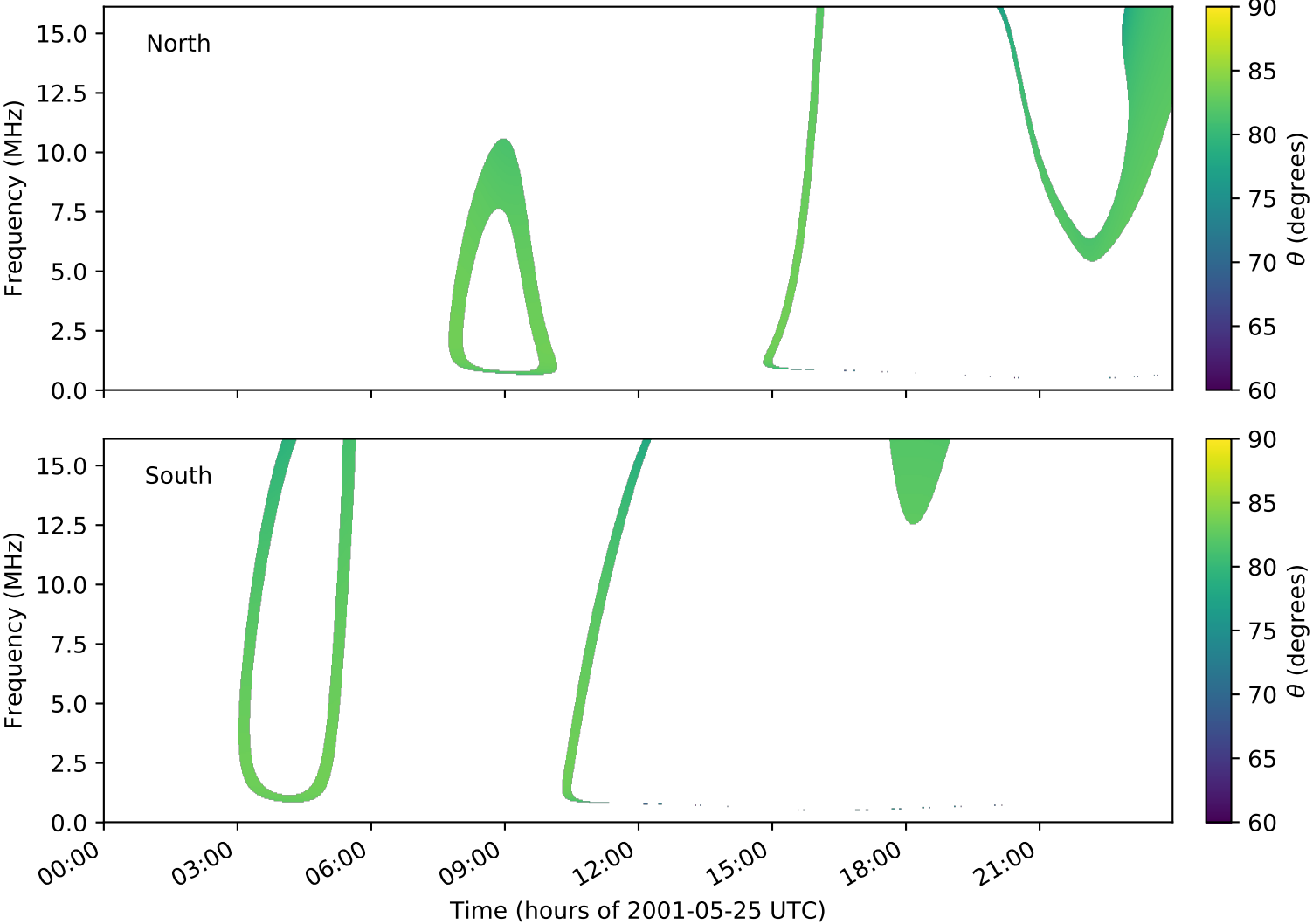
expres_cassini_jupiter_ganymede_isaac_lossc-wid1deg_3kev_20010525_v01.cdf
