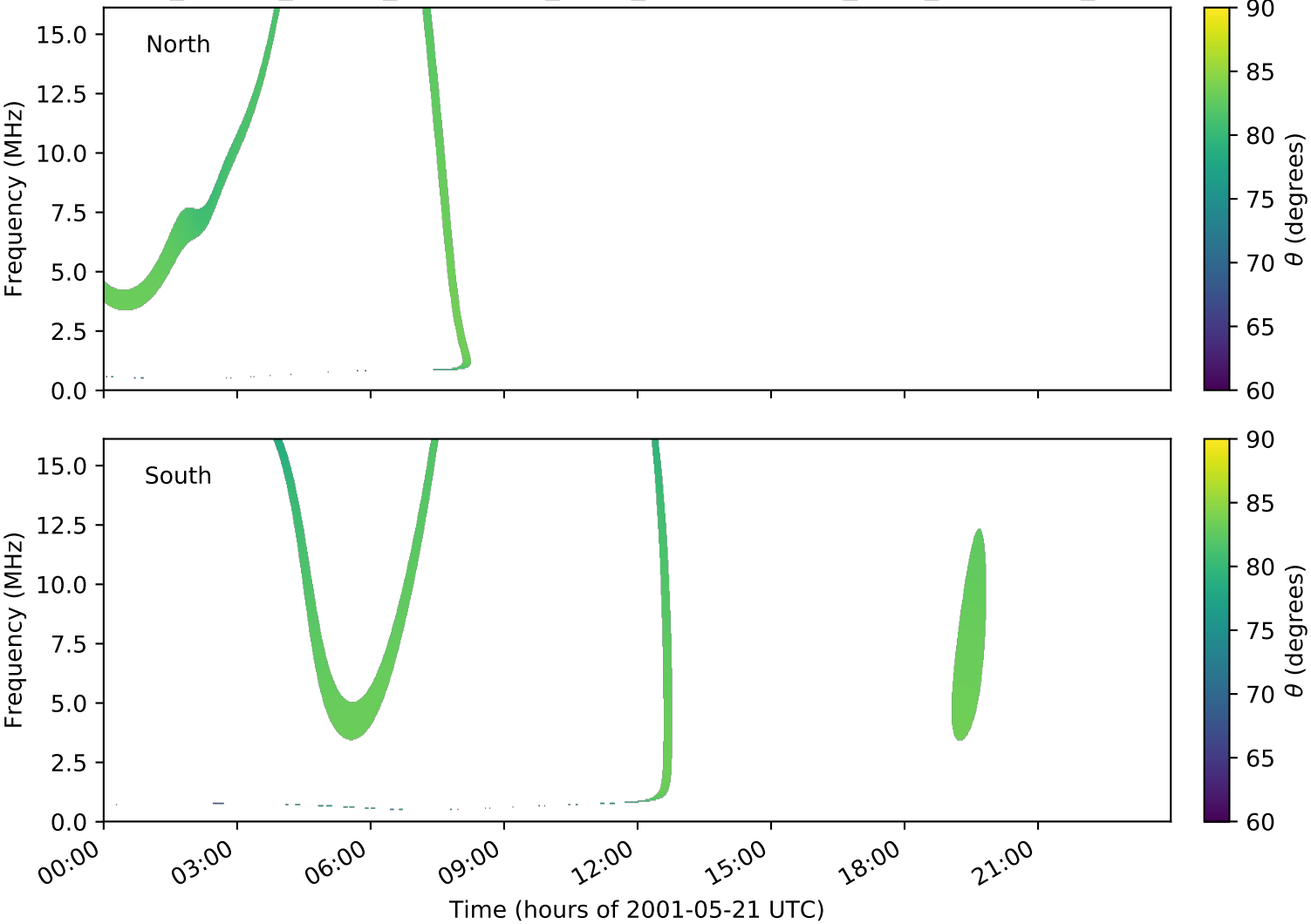
expres_cassini_jupiter_ganymede_isaac_lossc-wid1deg_3kev_20010521_v01.cdf
