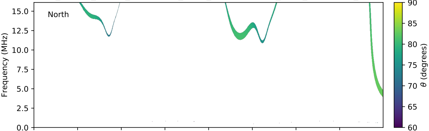
expres_cassini_jupiter_ganymede_isaac_lossc-wid1deg_3kev_20010520_v01.cdf
