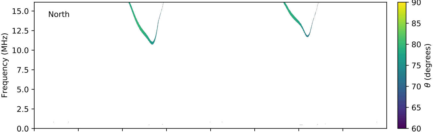
expres_cassini_jupiter_ganymede_isaac_lossc-wid1deg_3kev_20010519_v01.cdf
