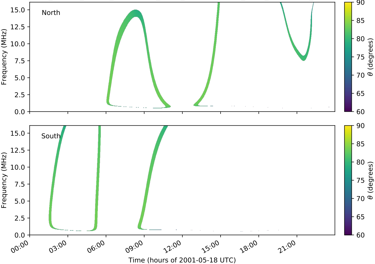
expres_cassini_jupiter_ganymede_isaac_lossc-wid1deg_3kev_20010518_v01.cdf
