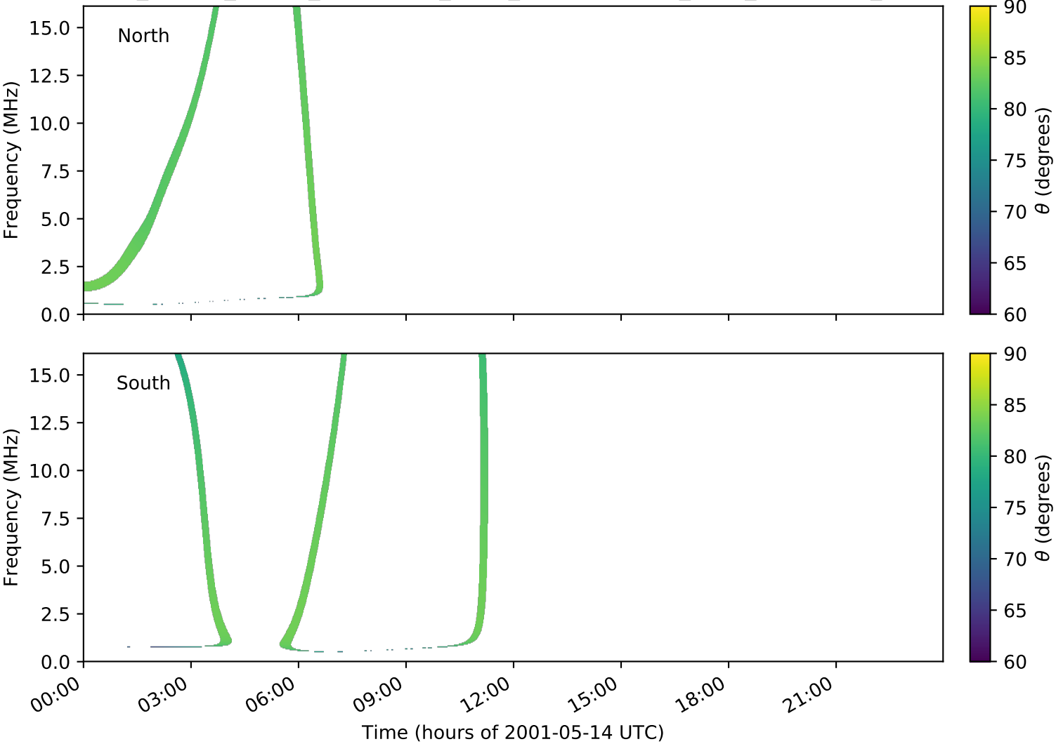
expres_cassini_jupiter_ganymede_isaac_lossc-wid1deg_3kev_20010514_v01.cdf
