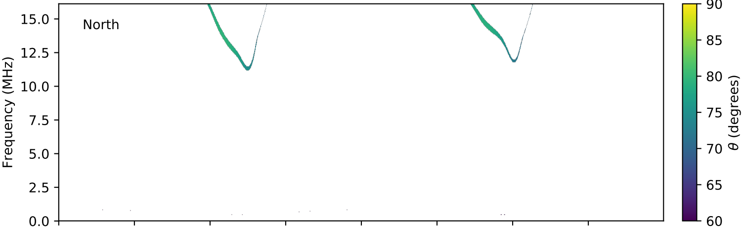
expres_cassini_jupiter_ganymede_isaac_lossc-wid1deg_3kev_20010512_v01.cdf
