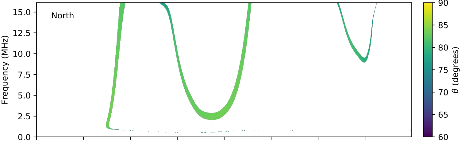
expres_cassini_jupiter_ganymede_isaac_lossc-wid1deg_3kev_20010511_v01.cdf
