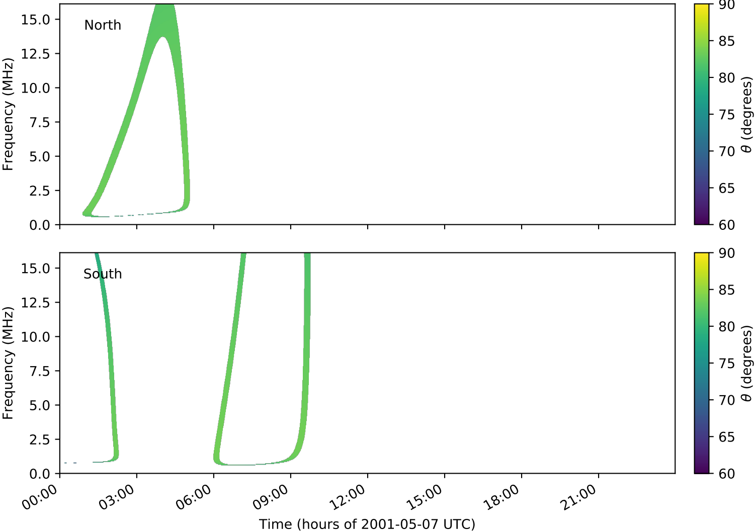
expres_cassini_jupiter_ganymede_isaac_lossc-wid1deg_3kev_20010507_v01.cdf
