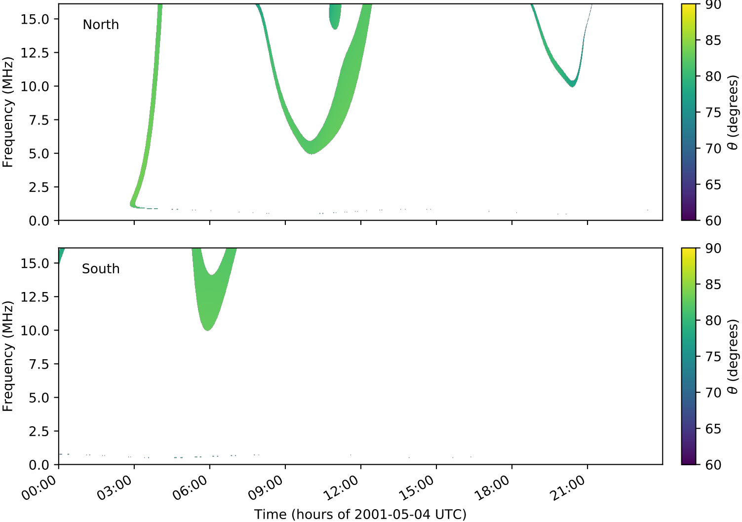
expres_cassini_jupiter_ganymede_isaac_lossc-wid1deg_3kev_20010504_v01.cdf
