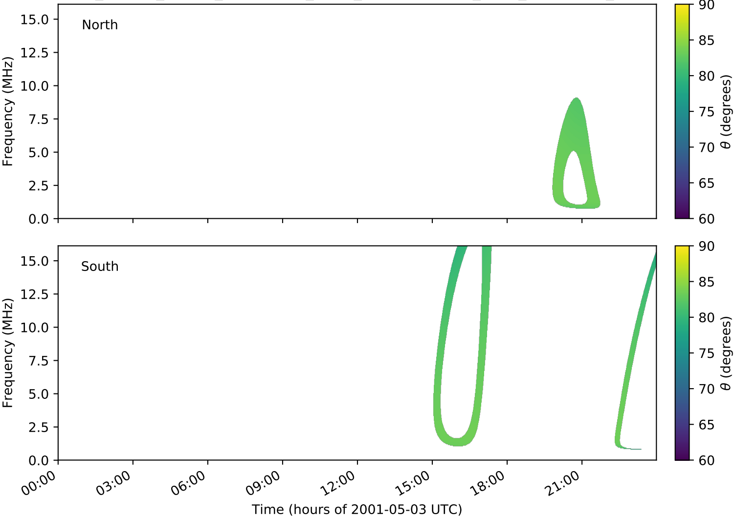
expres_cassini_jupiter_ganymede_isaac_lossc-wid1deg_3kev_20010503_v01.cdf
