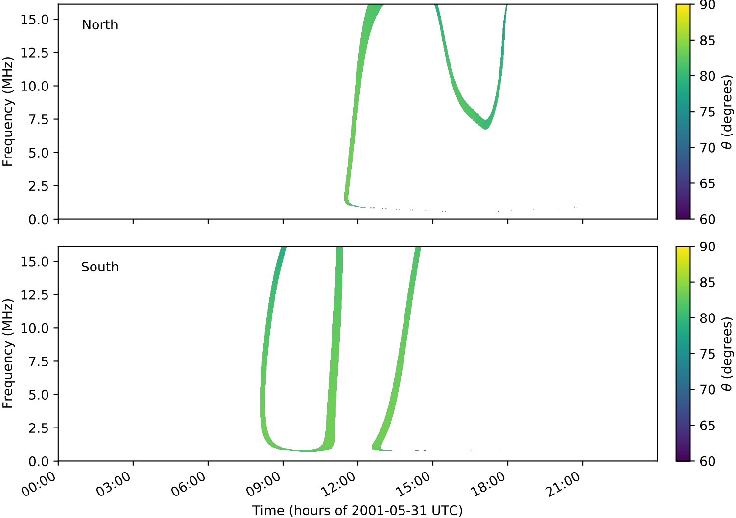
expres_cassini_jupiter_europa_isaac_lossc-wid1deg_3kev_20010531_v01.cdf
