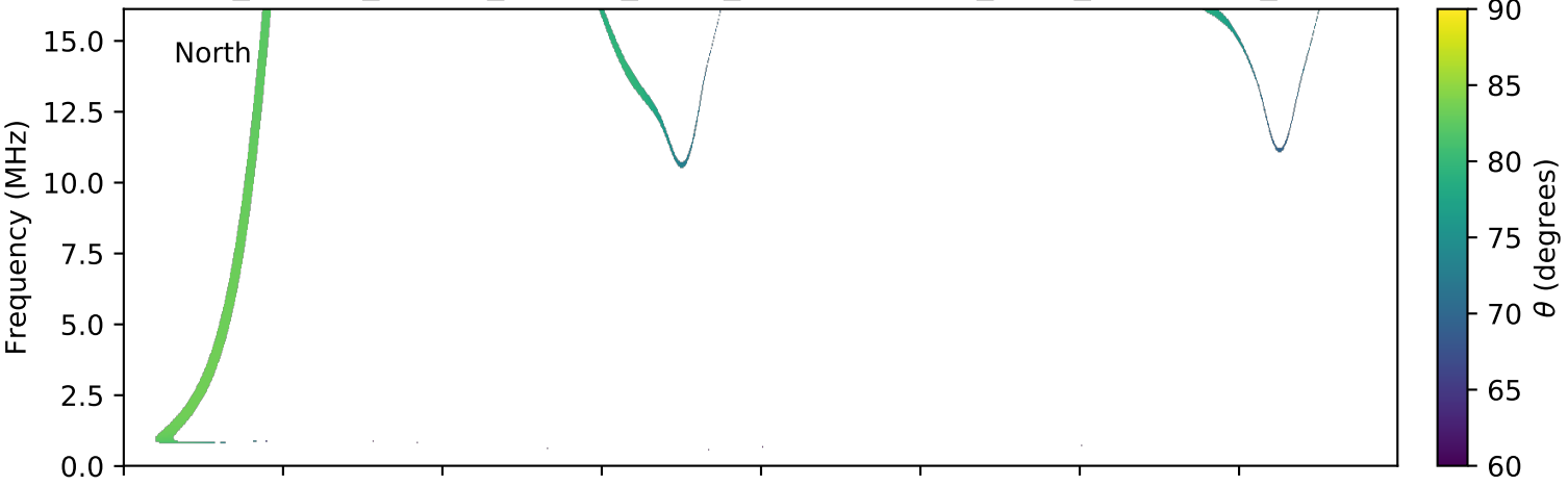
expres_cassini_jupiter_europa_isaac_lossc-wid1deg_3kev_20010528_v01.cdf
