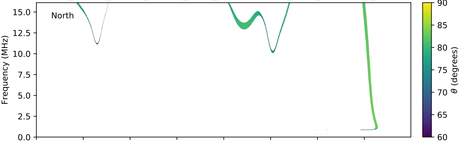
expres_cassini_jupiter_europa_isaac_lossc-wid1deg_3kev_20010525_v01.cdf
