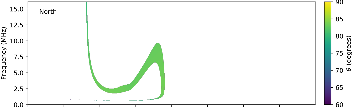
expres_cassini_jupiter_europa_isaac_lossc-wid1deg_3kev_20010522_v01.cdf
