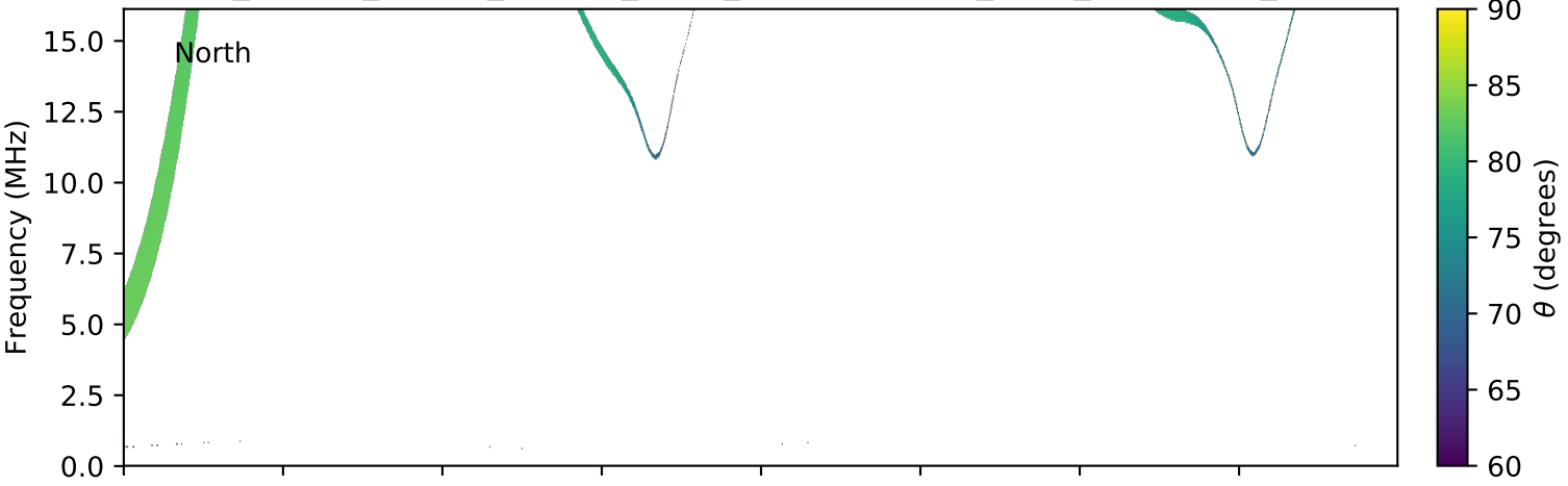
expres_cassini_jupiter_europa_isaac_lossc-wid1deg_3kev_20010521_v01.cdf
