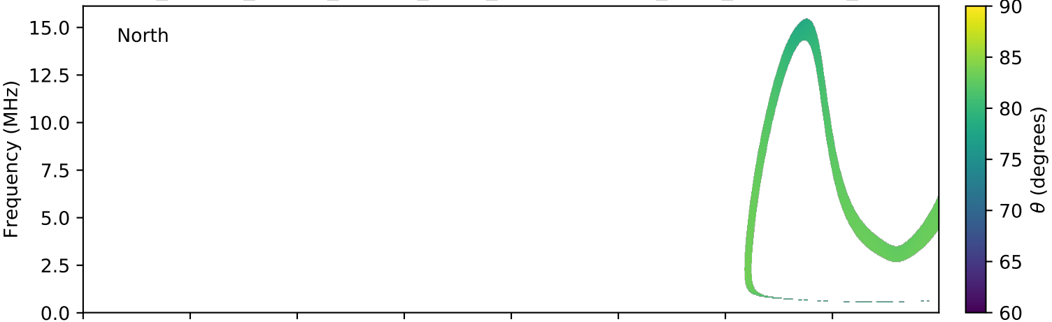
expres_cassini_jupiter_europa_isaac_lossc-wid1deg_3kev_20010520_v01.cdf
